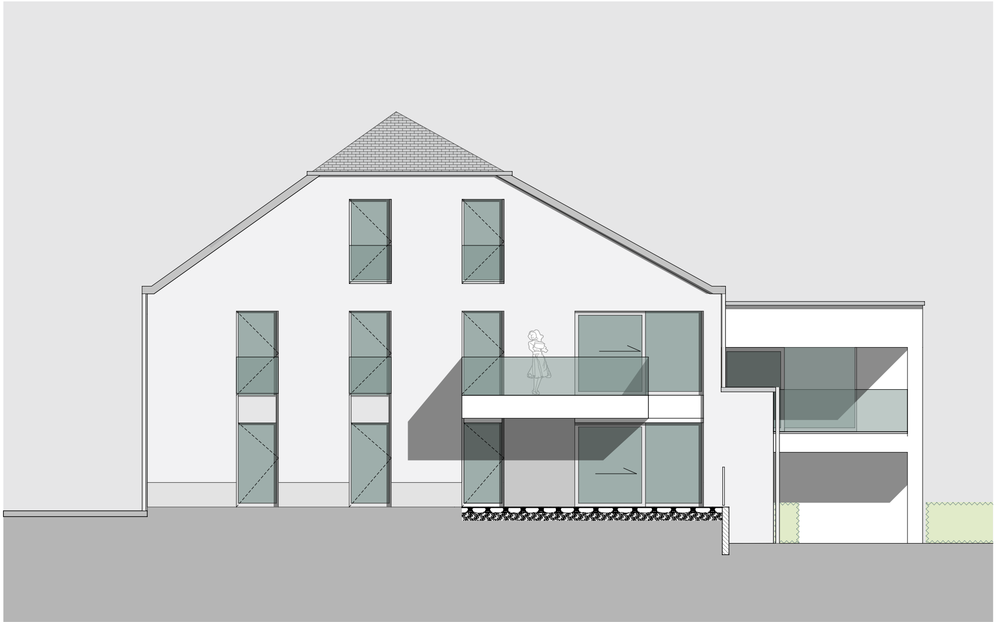
FACADE PIGNON 1:100
